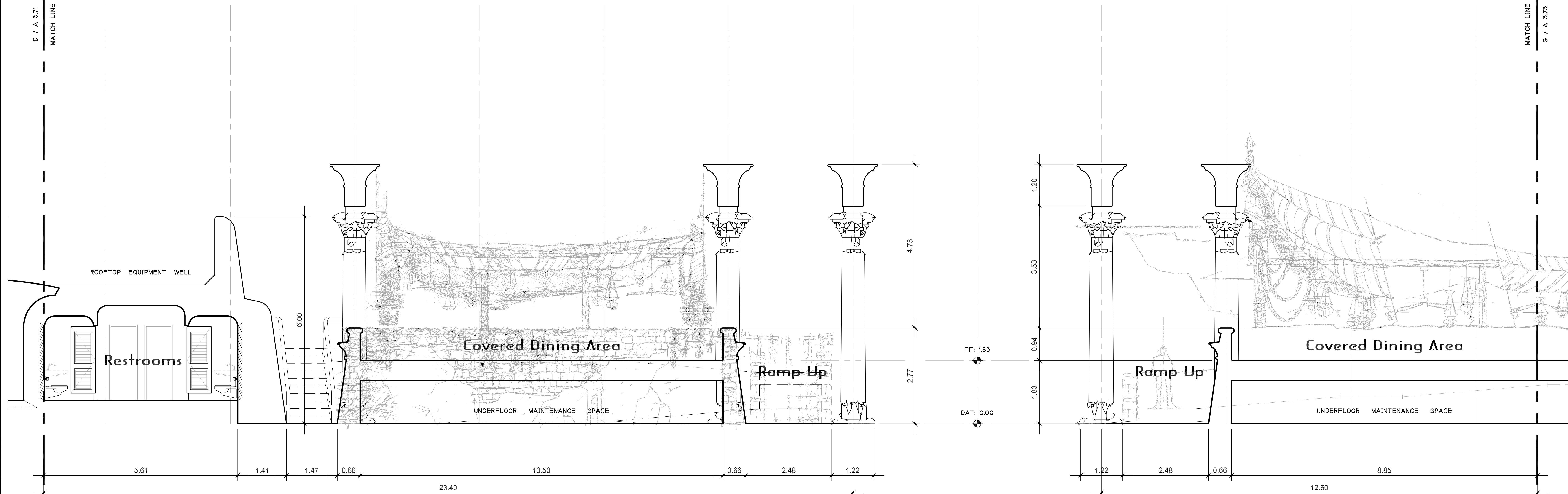
A Area 1 - Interior Elevation West SCALE = 1 : 50
